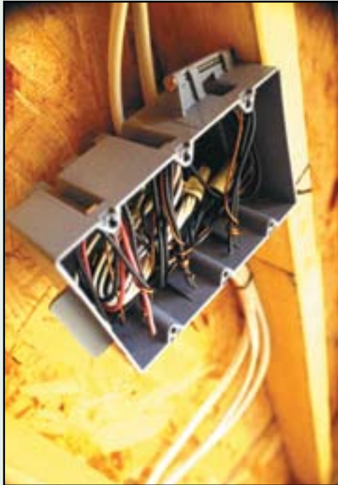
Black and red wires are usually energized, and white wires are usually neutral.
